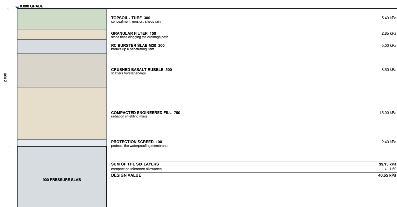
THE ENGINEERED COVER - 2 000 mm IN SIX LAYERS
