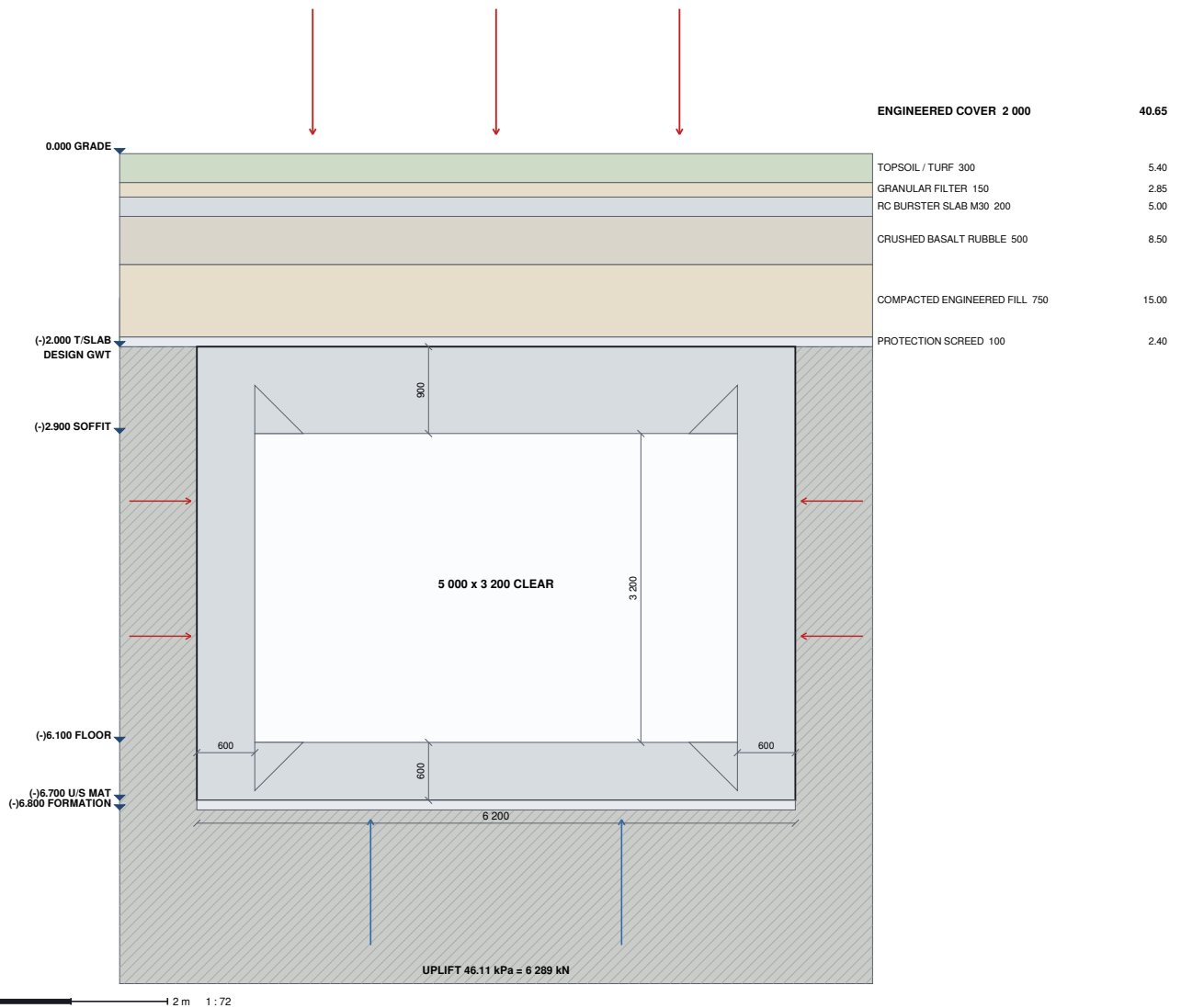
Fig 3.3 : Transverse Section through the Box
